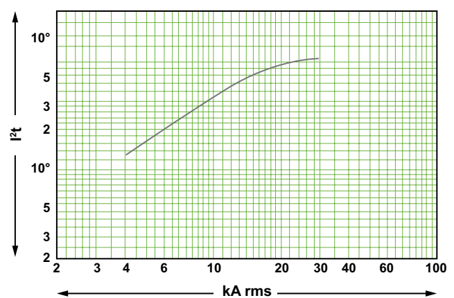
I²t Curve Curva I²t
